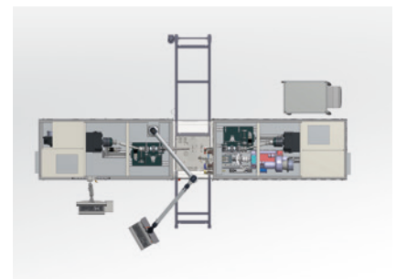
Layout with input and output right/left L = 5600 mm | W = 1100 mm
