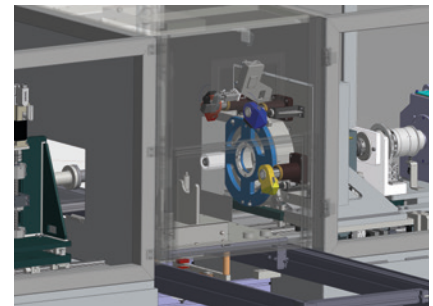
Test area with conveyor and transmission clamping
