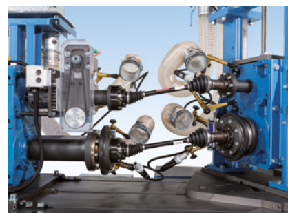
Test specimen and slave shaft in process
