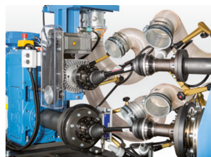
Cooling of the joints and non-contact temperature measurement
