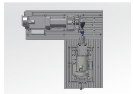
Total view of the test stand
