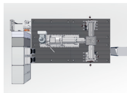
Possible T arrangement of the brake units
